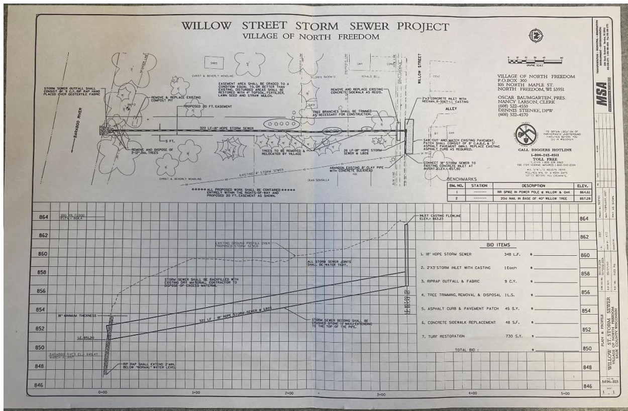
*Original engineering plan from MSA
